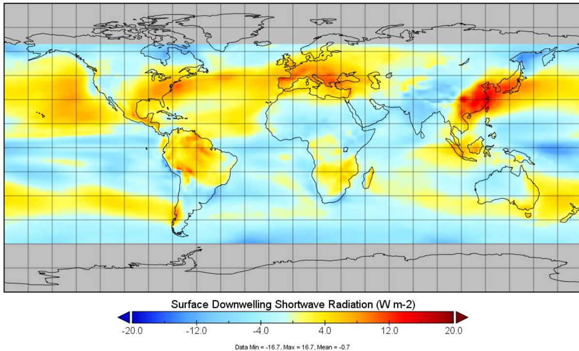
Fig. 3.2.1: Anomalies of global radiation in W/m 2 compared to 1996 - 2015 for the period 2080–2099 with IPCC scenario RCP8.5. Note that the unit is different than in the table above. For a yearly sum in kWh/m 2 , a factor of 8.76 has to be applied.
