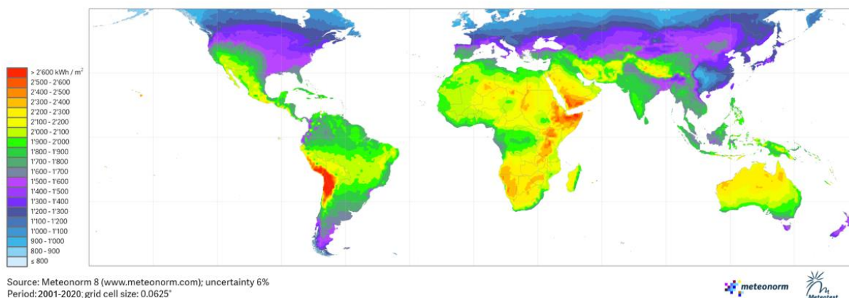
Fig. 3.1.2: Map of yearly sum of global irradiation in kWh/m 2 based on satellite and ground information. Means adapted mainly to the period 2001–2020.
