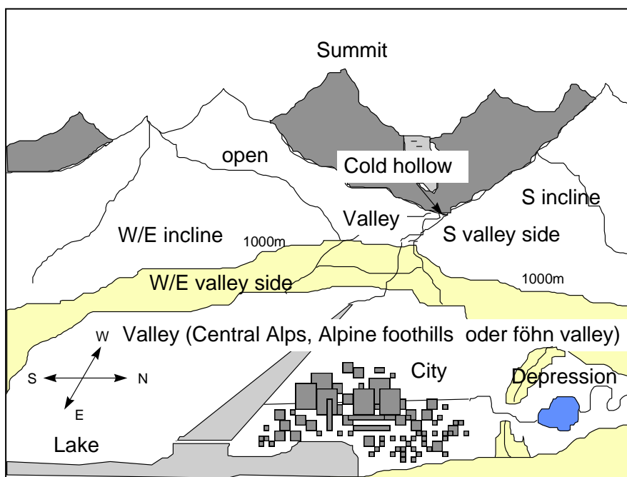
Fig. 2.4.1: Classification of the 14 types of terrain situations.
